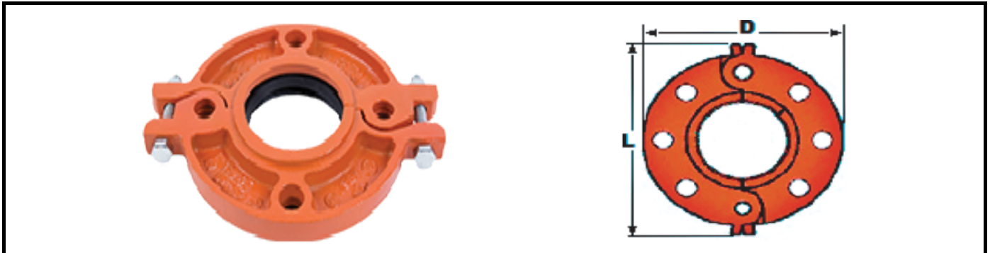
FLANGE ADAPTER - UL / FM PRESSURE 175 PSI - ANSI PRESSURE 150 PSI
